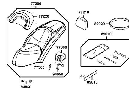
F9 座墊 -81- Seat
